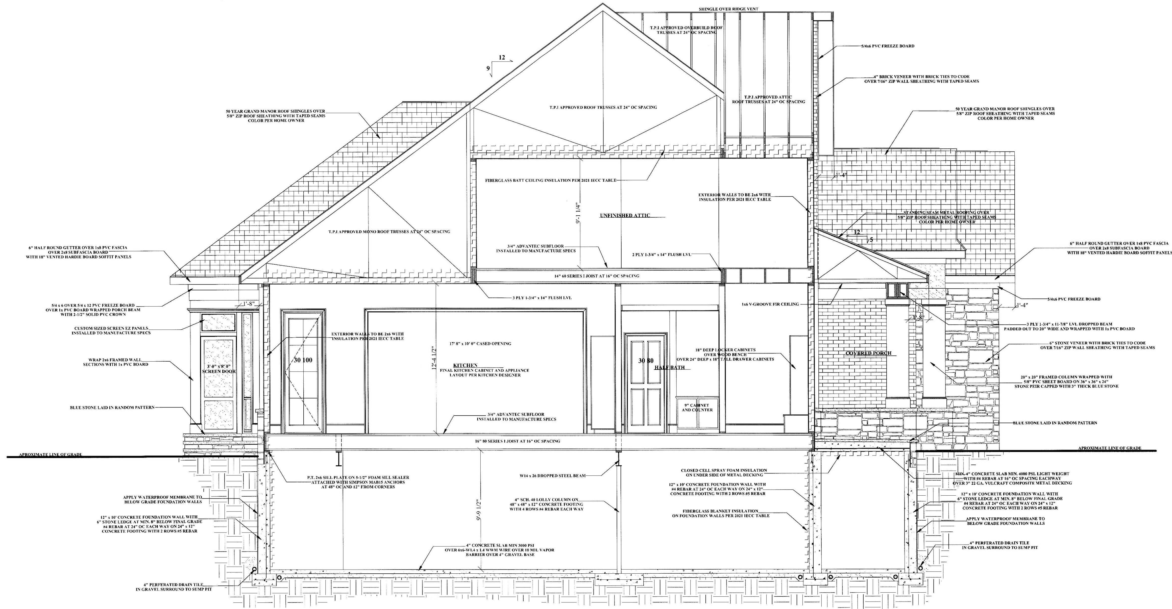
SECTION 1-C
